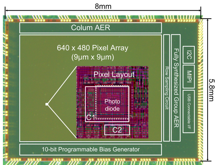
Figure 4.1.7: Micrograph of DVS chip in BSI process.
