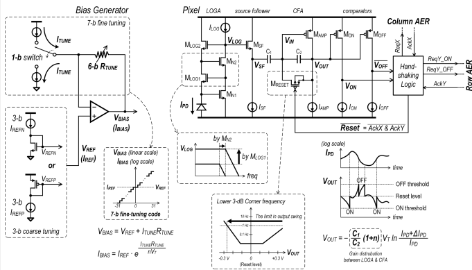
Figure 4.1.1: Pixel and bias generator.
