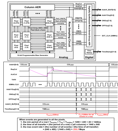
Figure 4.1.2: DVS architecture and timing diagram.
